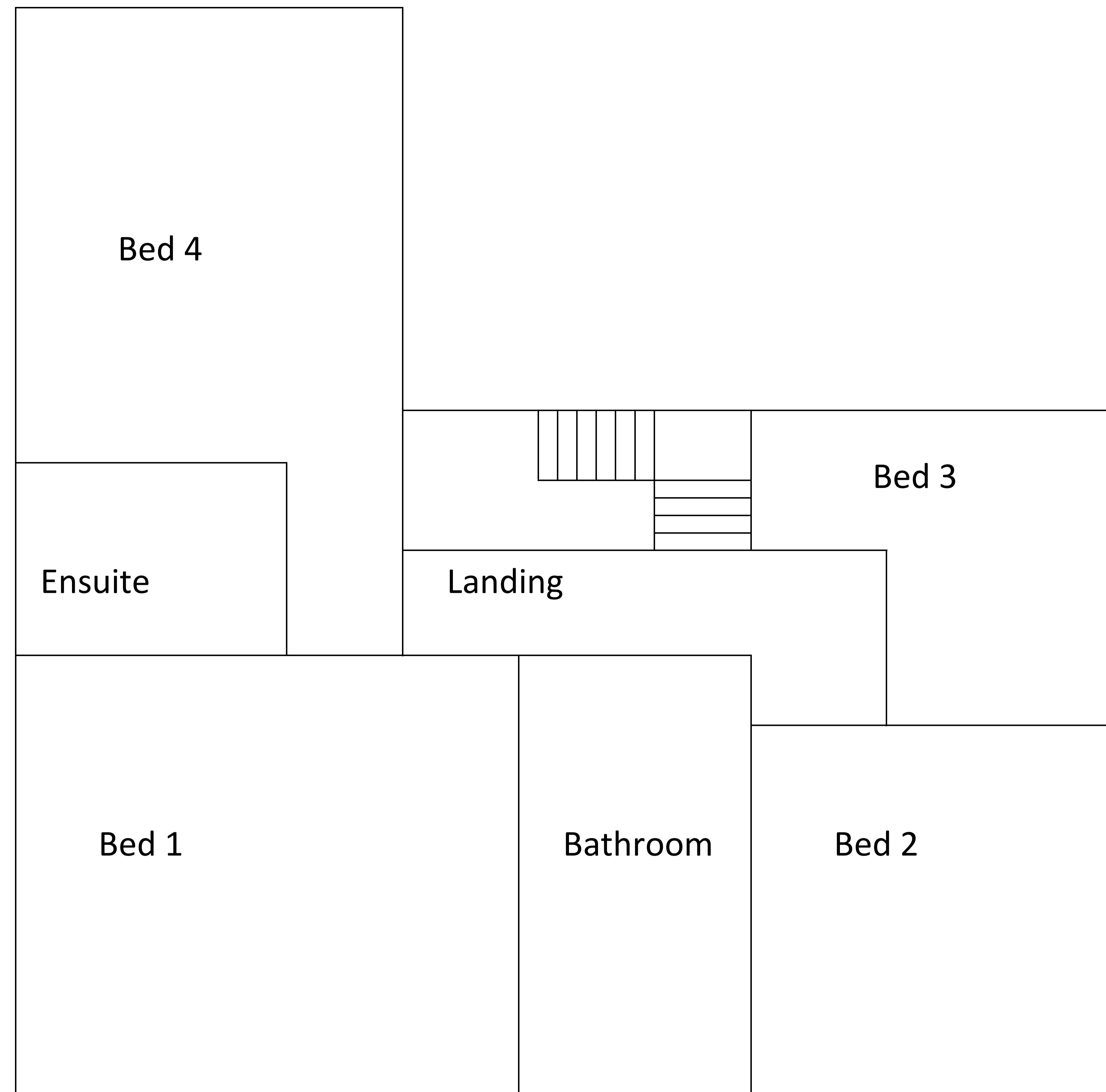
22 HAMPSON WAY: FIRST FLOOR PLAN
